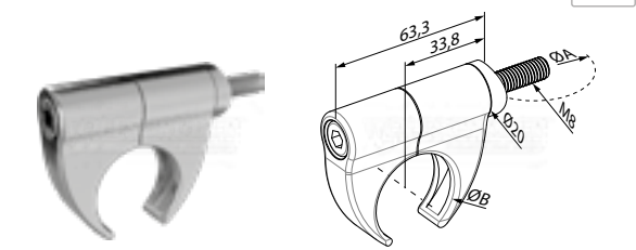
support de tube (info 1)
