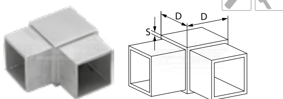
raccord coudé 90°
