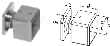
embase murale sans platine (info 1)
