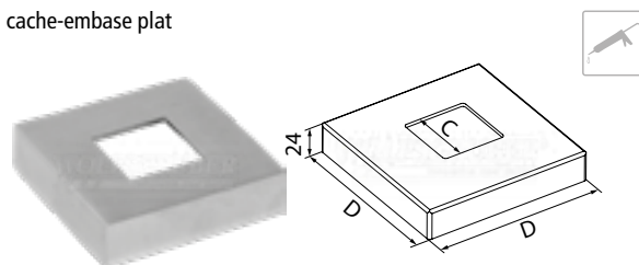
cache-embase plat
