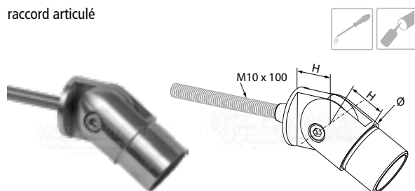
raccord articulé
