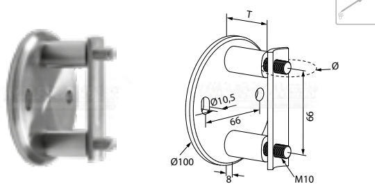
fixation murale
