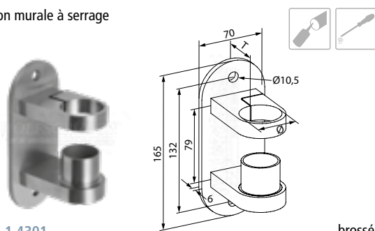
fixation murale
