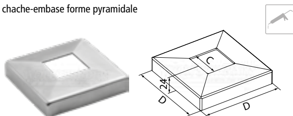
cache-embase forme pyramidale
