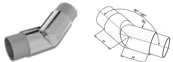
raccord orientable (info 3)
