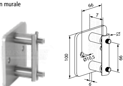
fixation murale
