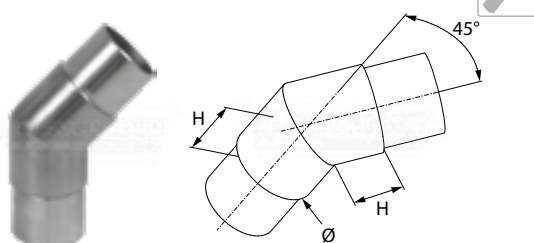
raccord coudé 45°
