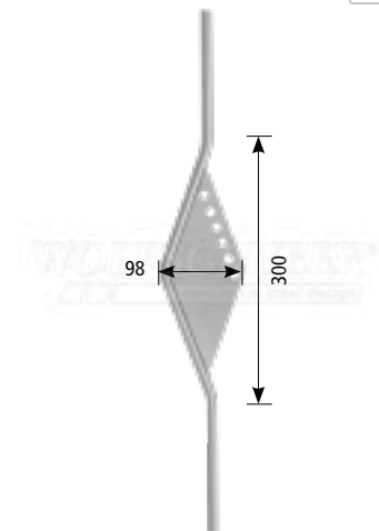
barreau Ø12x1000
