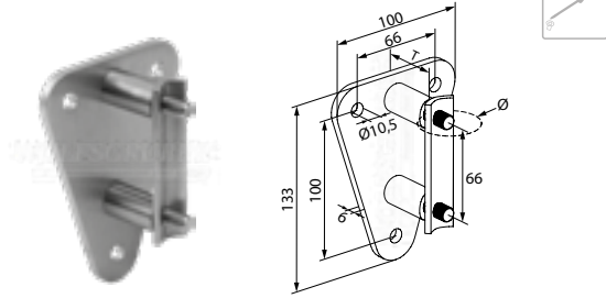
fixation murale
