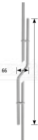
barreau Ø12x1000
