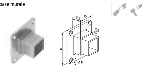
embase murale
