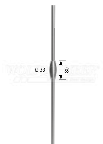
barreau Ø12x1000
