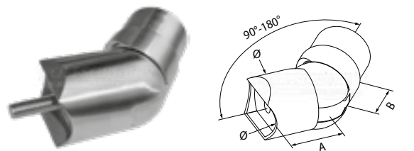
raccord articulé (info 1)
