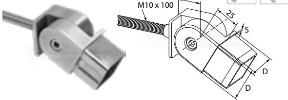
raccord articulé
